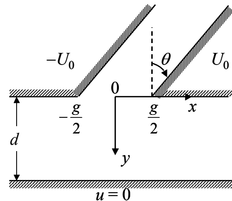
Fig. 1. Two-dimensional geometry of the asymmetrical head, with gap length g and exterior corner inclination angle \theta . The poles are assumed to have infinite permeability and therefore with equipotentials \pm U_0 , at a distance d from a soft magnetic underlayer (SUL) held at zero potential. To model two-dimensional heads without an underlayer, the SUL is removed with d \rightarrow \infty .
