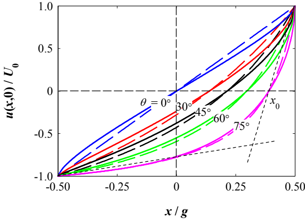
Fig. 2. Calculated gap surface potential using finite-elements (solid lines) and the approximate surface potential in (2) and (3) (dashed lines) for different corner angles. The dotted straight lines highlight the approximate hyperbolic locus of the asymmetrical potential, and were used as guides to derive the rational function approximation for the potential.
