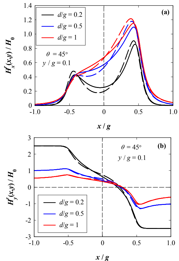
Fig. 10 (a) Normalised x field component, and (b) y field component for the asymmetrical head in the presence of a SUL, for exterior corner angle \theta = 45^\circ . Solid lines are for the finite-element calculations, and the dashed lines are from the theoretical model in (22) and using the surface field from (23).
