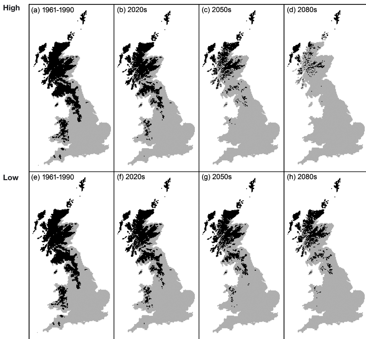
Fig. 3. Area covered by the bioclimatic envelope of blanket peatlands predicted by PeatStash using the bioclimatic thresholds associated with the 1961–1990 baseline climate for the UKCIP02 high and low emissions scenarios ('High' and 'Low', respectively) for 3 time periods: 2020s, 2050s and 2080s. An Ordnance Survey/EDINA supplied service (© Crown Copyright/database 2009) and Met Office/UKCIP gridded climate data (UKCIP02 © Crown Copyright 2002)
