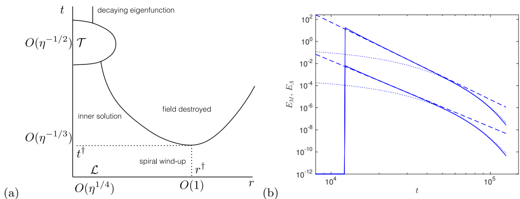
FIGURE 3. (a) Schematic of kinematic evolution of magnetic field for \eta \ll 1 , and (b) log-log plot of E_M (upper solid) and E_A (lower solid) as functions of time t . In (b) the scaling laws t^{-7} (4.10) and t^{-6} (4.11) are depicted (dashed), and the formulae (4.13), (4.14) are shown (dotted).
