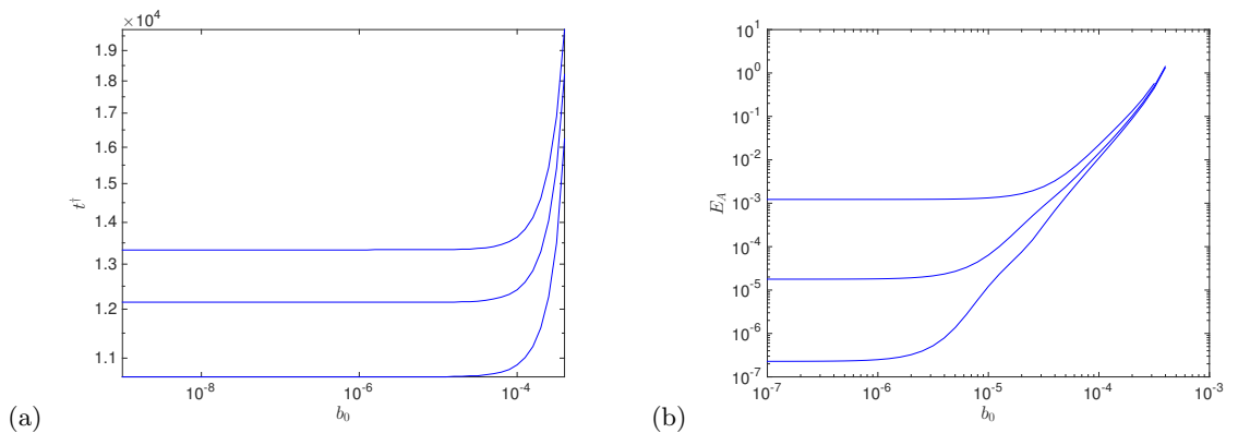
FIGURE 9. (a) The onset of flux expulsion t^\dagger as a function of initial field strength b_0 using different thresholds \delta = 10^{-4}, 10^{-3} , and 10^{-2} , reading down the curves. (b) E_A plotted against b_0 at times \frac{1}{2}\mathcal{T}, \mathcal{T} and 2\mathcal{T} , reading down the curves.
