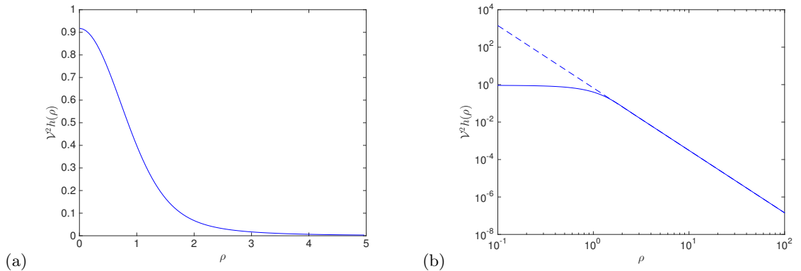
FIGURE 11. Plot of \mathcal{V}^2 h(\rho) (solid) given in (4.36) against \rho with (a) linear scales, (b) log–log scales. In (b) the approximation (4.37) is shown dashed.
