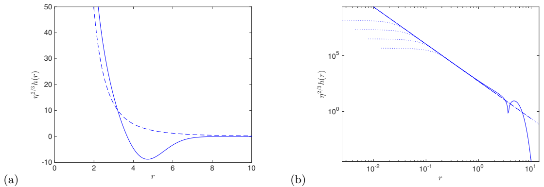
FIGURE 12. Plot of \eta^{2/3} h(r) (solid) given in (4.32) for the Gaussian vortex against r with (a) linear scales, (b) log–log scales (taking the absolute value). In (a) the approximation (4.33) is shown dashed: it is also present in (b) but is somewhat overlapped with dotted curves showing \eta^{2/3} h(\rho) from (4.36) plotted against r for \eta = 10^6 to 10^9 , reading up the curves.
