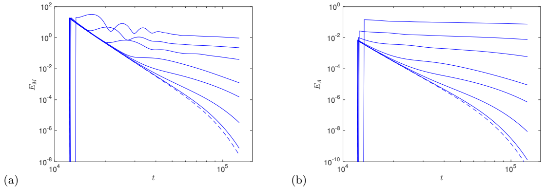
FIGURE 8. Plotted are (a) the magnetic energy E_M and (b) E_A as functions of time t for varying field strength b_0 . The dashed curves are kinematic traces, while b_0 = 2 \times 10^{-4}, 10^{-4}, 5 \times 10^{-5}, 2 \times 10^{-5}, 10^{-5}, 5 \times 10^{-6} and 2 \times 10^{-6} , going down the curves on the right of the plots.
