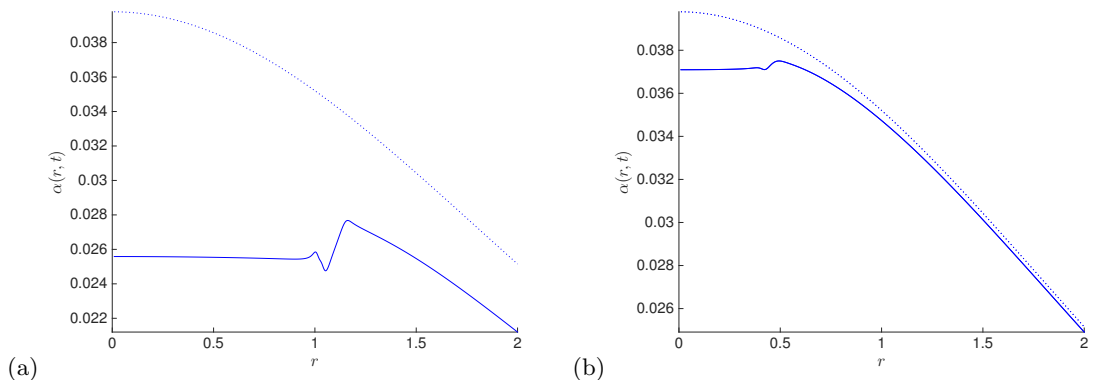
FIGURE 6. Final angular velocity profiles for (a) b_0 = 2 \times 10^{-4} in figure 5 and (b) 5 \times 10^{-5} in figure 7, for t = 5 \times 10^4 . The function \alpha(r, t) (solid) is plotted against r , with the initial profile \alpha(r, 0) shown dotted.
