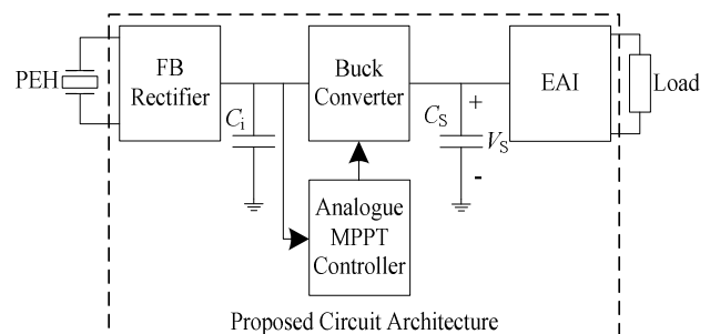
Fig. 2. Proposed batteryless power management circuit.
