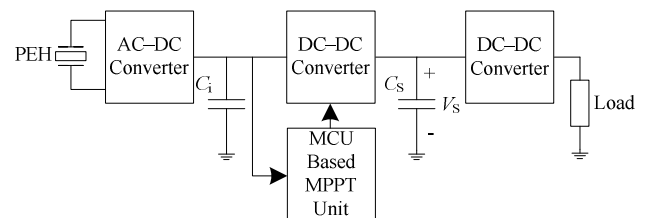
Fig. 1. Conventional two-stage power management circuit for batteryless system.
