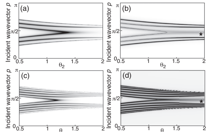
FIG. 2. (a) Reflected intensity as a function of wave vector for opacity parameters \theta_1 = 1 and varying \theta_2 . (b) Time delay as a function of wave vector and \theta_2 ; the Lorentzian feature indicative of the topological mode for \theta_2 > \theta_1 is indicated with a *. Corresponding plots are shown for 6.5 units in (c) and (d).
