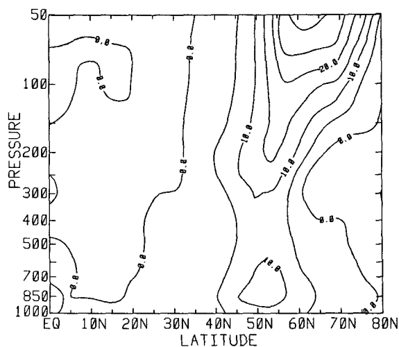
FIG. 5. As in Fig. 4 but by stationary waves.
