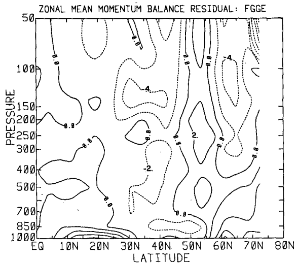
FIG. 10. Momentum balance residual for FGGE data. Contour interval of 2 \text{ m s}^{-1} (\text{day})^{-1} . Negative values indicate that negative acceleration (drag) is needed to complete the momentum balance.
