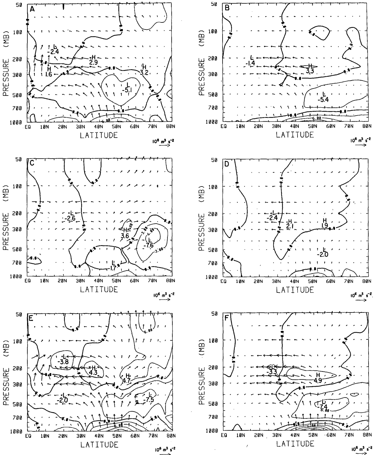
FIG. 6. Eliassen-Palm diagrams for FGGE 58-day mean and Oort 90-day mean winter data. EP flux divergence contour interval of 3 \text{ m s}^{-1} (\text{day})^{-1} . See text for scaling of arrows. (a) FGGE data, transient eddies, (b) Oort data, transient eddies, (c) FGGE data, stationary waves, (d) Oort data, stationary waves, (e) FGGE data, total waves, (f) Oort data, total waves.
