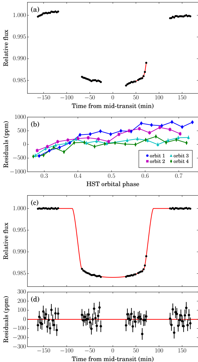
FIG. 1.— HST /WFC3 G141 white transit lightcurve for WASP-121b. (a) Raw flux time series, with solid lines indicating the predictive mean of the maximum likelihood GP model. (b) Residuals after removing the transit and linear time trend, which correlate with HST phase and dispersion drift. (c) Relative flux as a function of time after removing the linear time trend and systematics component of the GP model, with solid line indicating the inferred transit signal. (d) Residuals as a function of time with photon noise errorbars after removing the combined transit, linear time trend, and GP systematics model.
