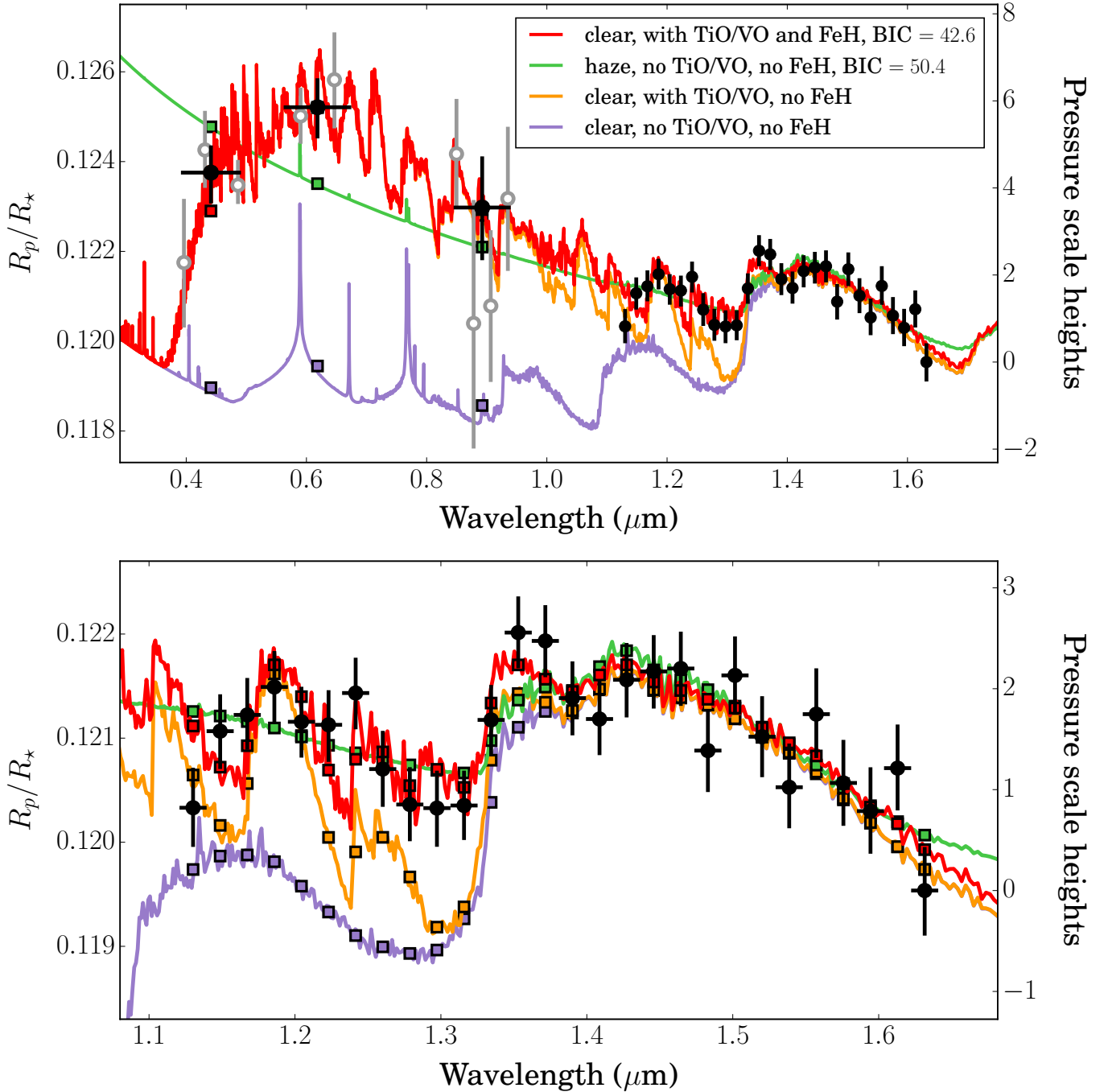
FIG. 3.— Measured transmission spectrum for WASP-121b, with models. In the top panel, unfilled gray data points show results for fits to individual photometric lightcurves, with horizontal offsets applied for clarity, and filled black data points show results for joint fits to all lightcurves in the corresponding bandpass. The lower panel shows a zoomed-in view of the WFC3 transmission measurements. Models assume solar abundances and chemical equilibrium, with the exception of TiO, VO, and FeH, the abundances of which were adjusted to fit the data. (Red line) Clear atmosphere including TiO, VO, and FeH opacity. (Orange line) Same as previous, but excluding FeH opacity to illustrate its effect. (Green line) Hazy atmosphere with enhanced Rayleigh scattering, excluding TiO, VO, and FeH opacity. (Purple line) Clear atmosphere excluding TiO, VO, and FeH opacity.
