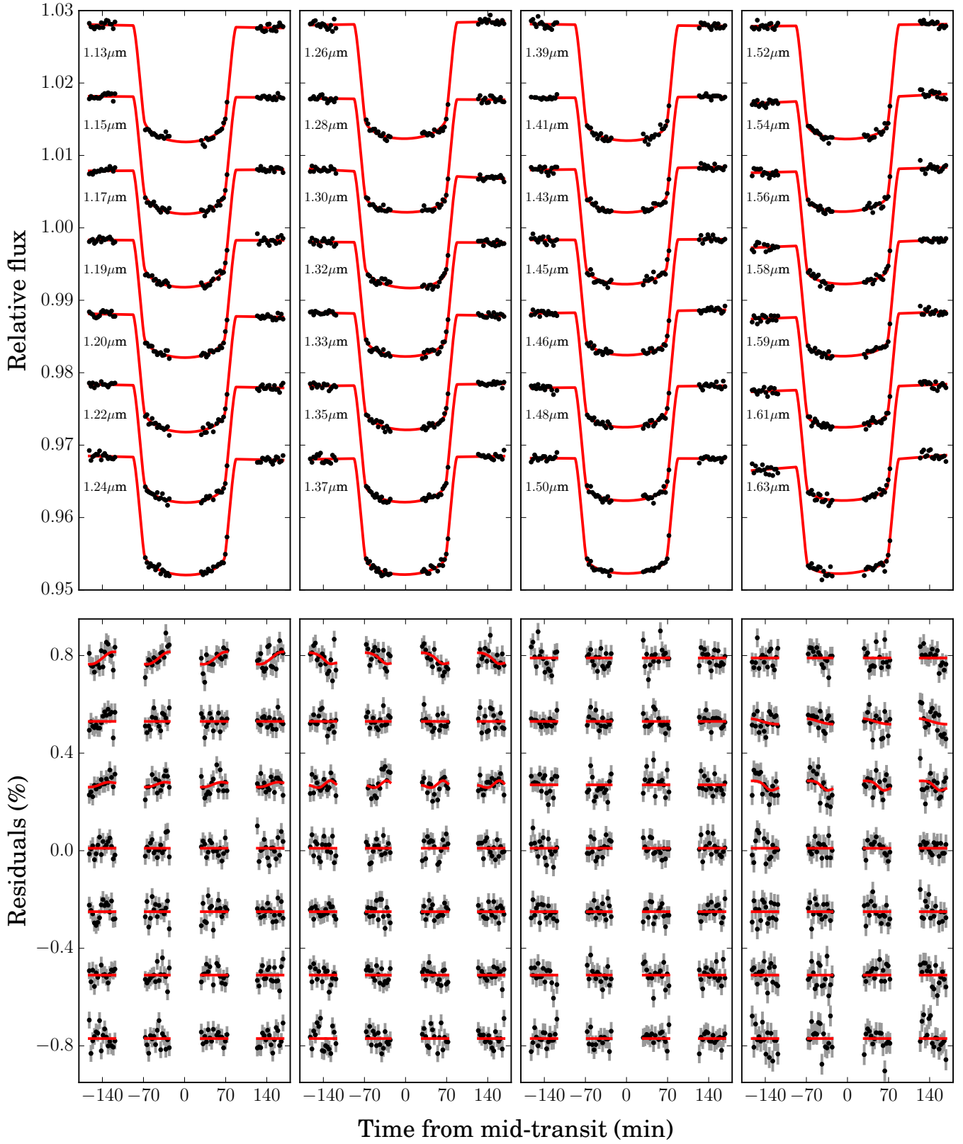
FIG. 2.— (Top) Raw spectroscopic lightcurves with solid lines showing best-fit transit signals multiplied by linear time trends. (Bottom) Model residuals with photon noise errorbars in gray and solid lines showing GP model fits. Note that the transit signals, linear time trends, and GP systematics models were fit simultaneously in practice, but have been separated here for illustrative purposes.
