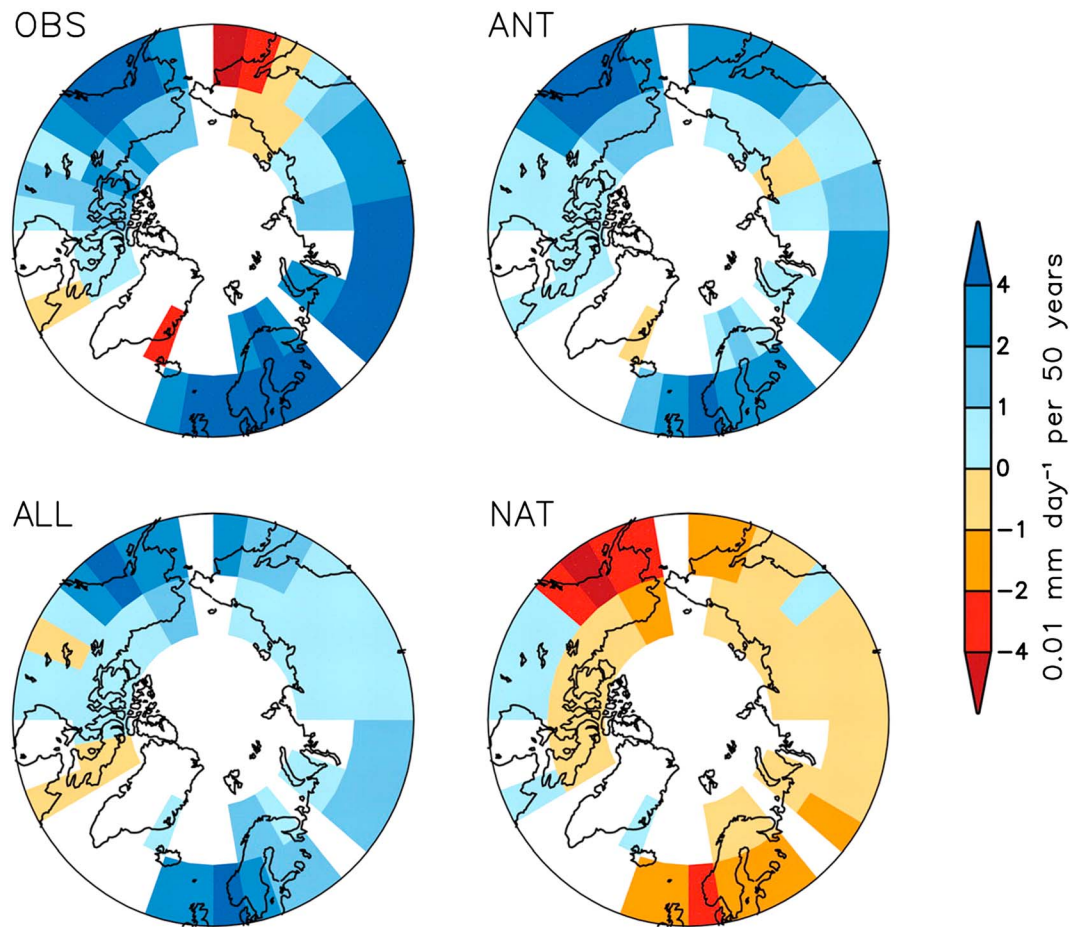
Figure 4. Large-scale precipitation trends ( 0.01 \text{ mm d}^{-1} per 50 years) during 1950 to 1999 based on observations (OBS) and CMIP3 model simulations driven by different forcings: anthropogenic (ANT; greenhouse gases and sulfate aerosols), natural (NAT; solar and volcanic), and both of them (ALL). Areas with less than 40 years of observations are marked with white space. Reproduced with permission from Min et al. [2008].
