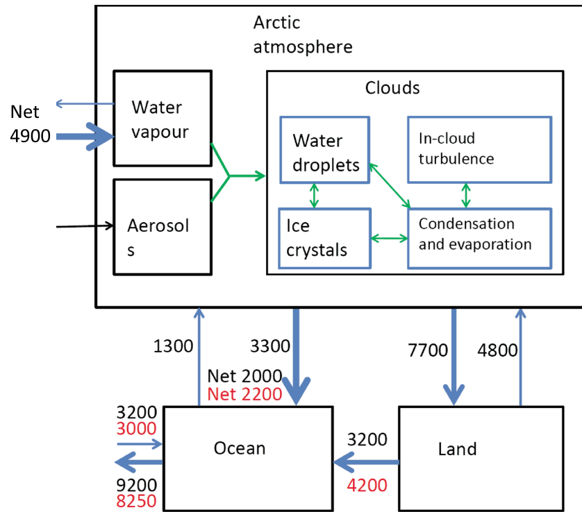
Figure 1. Schematic presentation of the main freshwater components and processes in the Arctic atmosphere. The numbers in black indicate the freshwater transports in \text{km}^3/\text{yr} on the basis of Serreze et al. [2006], representing the period of 1979–2001, whereas the numbers in red are estimated for the period 2000–2010 by Haine et al. [2015].
