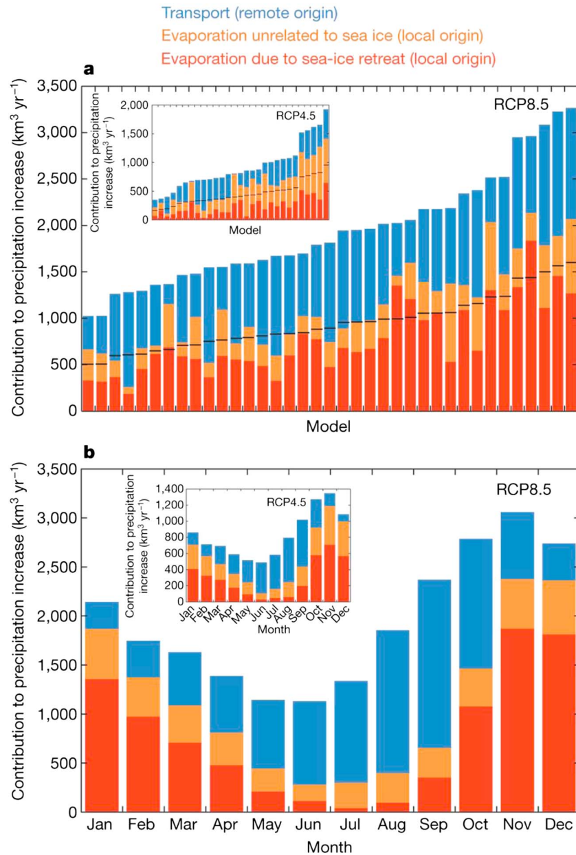
Figure 6. Simulated annual and monthly 21st century changes in Arctic mean precipitation, poleward moisture transport across 70°N (remote origin), and surface evaporation components (local origin). (a) Annual mean changes, where each bar denotes one CMIP5 model sorted according to the magnitude of the simulated precipitation change (horizontal black lines represent 50% of each column). (b) Seasonal changes, where each bar represents the monthly and multimodel mean. Changes are given for the strong (RCP8.5) and intermediate (insets, RCP4.5) forcing scenarios. The total Arctic surface evaporation (the sum of the red and orange bars) is separated into its ice retreat (red) and non-ice retreat (orange) components. The attribution of sea ice retreat to the total surface evaporation was evaluated by calculating monthly evaporative flux differences over only the ice retreat regions, which were then summed over the respective 10 year periods. Reproduced with permission from Bintanja and Selten [2014].
