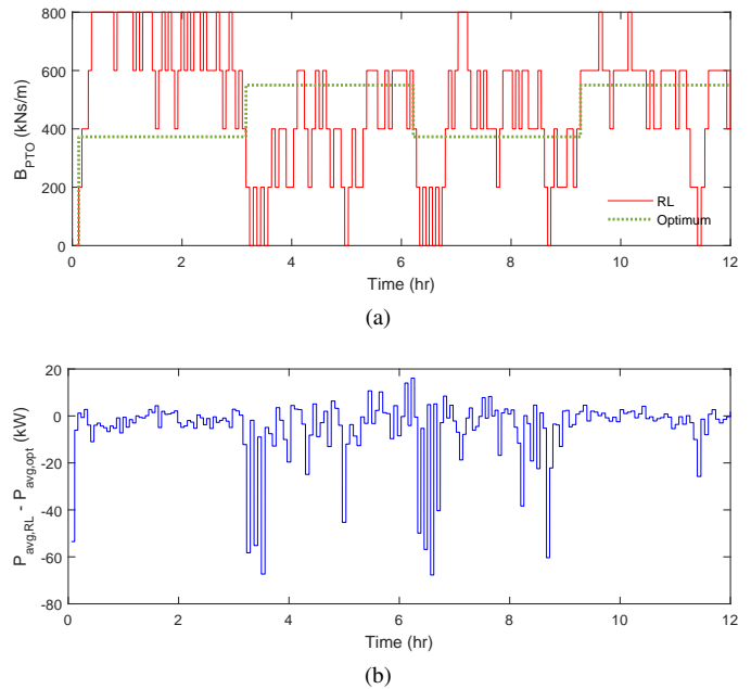
Fig. 12. Optimal and RL-control-selected ( J = 1, K = 4, L = 5 ) PTO damping coefficient (a) and corresponding mean absorbed power (b) in irregular waves with four sea states, generated from the combination of H_s = 2, 3 m and T_z = 7, 8 s.
