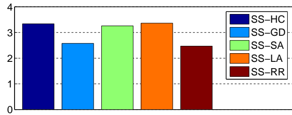
Figure 5: Comparisons of the different move acceptance methods when combined with the sequence-based selection method. The vertical axis shows the score values using ITC 2011 ranking strategy over 10 runs from eight instances
