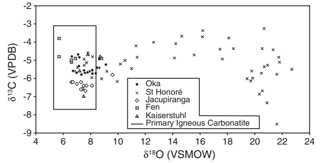
Fig. 3. Carbonatite C and O analyses from Oka (Deines, 1989; Haynes et al., 2003), St Honoré (Deines, 1989), Jacupiranga (Morikiyo et al., 1990; Santos and Clayton, 1995; Haynes et al., 2003), Fen (Andersen, 1987), and Kaiserstuhl (Hubberten et al., 1988). Included for reference is the PIC field after Jones et al. (2013).
