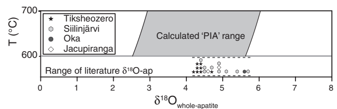
Fig. 2. Compilation of previous O-isotope analyses of apatite from Oka (Conway and Taylor, 1969), Jacupiranga (Santos and Clayton, 1995), Tiksheozero, and Siilinjärvi (Tichomirowa et al., 2006), plotted against an estimated PIA range using the PIC range (+5.3 to +8.4‰) and the fractionation factor from Fortier and Lüttge (1995) for the temperatures 600–700 °C.
