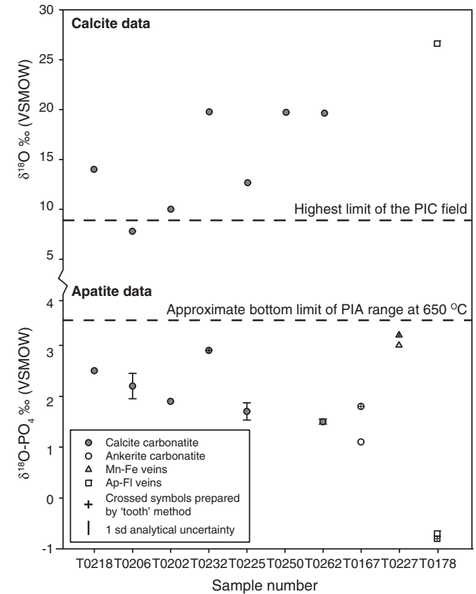
Fig. 7. Songwe \delta^{18}\text{O} results from calcite (above) and \delta^{18}\text{O} results from apatite (below), arranged in approximate paragenetic order. Error bars on apatite results represent replica values. Crossed symbols represent apatite results analysed by the 'tooth' method. Also included is the approximate bottom limit of the PIA and upper limit of the PIC field (Jones et al., 2013).
