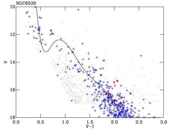
Figure 13. The photometry of NGC6530 from Prisinzano et al. (2005) (dots). Crosses are X-ray sources from Prisinzano et al. (2005). Circles are weak H\alpha stars from Sung et al. (2000). Asterisks are strong H\alpha stars from Sung et al. (2000).
