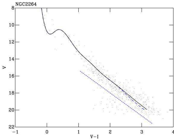
Figure 3. The effect of choosing a wider colour-magnitude selection in NGC2264. The effect is limited by the large number of sources within the sequence. The solid curve is the result using no selection, with the dotted line being the colour-magnitude selection and the dashed line the spline fit after the colour-magnitude selection is enforced i.e. only stars above the line were used to produce the spline curve.
