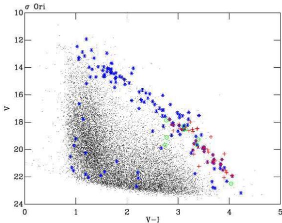
Figure A2. The full catalogue for the \sigma Ori field (dots). Circles are members from Burningham et al. (2005b), while asterisks are X-ray sources from Sanz-Forcada et al. (2004). Crosses are members from Kenyon et al. (2005).
