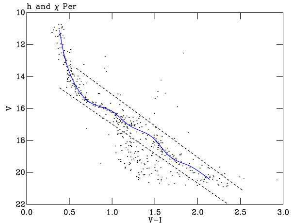
Figure 16. Stars within 2 arcmin radius of the centres of h and \chi Per. Stars in the h Per region have been shifted in extinction to match those \chi Per. The dotted lines are the colour-magnitude cuts used, and the solid curve the best fitting spline.
