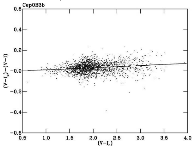
Figure 1. The difference in V - I for Cep OB3b between data taken in the system used here and using Cousins I filter. The line is the best fit through the data.
