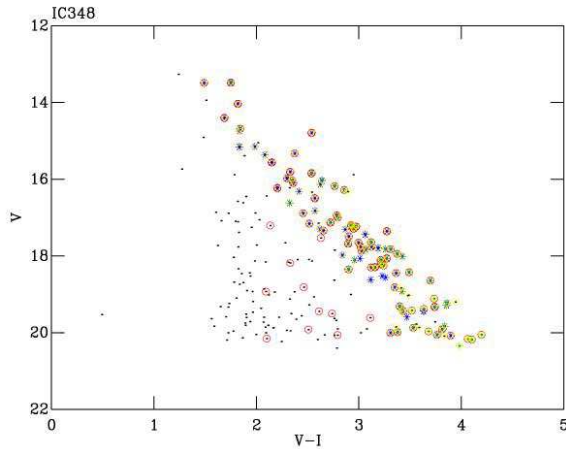
Figure A4. The full catalogue for the IC348 field (dots) The asterisks are X-ray sources from Preibisch & Zinnecker (2002) and the Second ROSAT PSPC catalogue. Circles are the periodic variables from Cohen et al. (2004) and Littlefair et al. (2005). Crosses are H\alpha sources from Herbig (1998). Triangles are spectroscopic members with extinctions from Luhman et al. (2003) and Herbig (1998).
