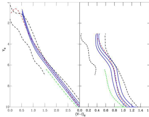
Figure 24. The sequence for Cep OB3b assuming three different distance moduli (solid lines). NGC2264, h and \chi Per, \sigma Ori, and the ONC are shown as dashed lines for reference.
