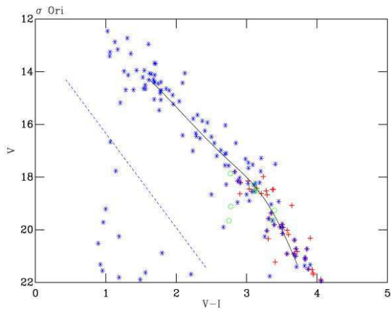
Figure 7. Stars selected as members in \sigma Ori. Circles are Burningham et al. (2005b) members. Asterisks are X-ray sources from Sanz-Forcada et al. (2004). Crosses are members from Kenyon et al. (2005). The fitted spline curve is shown. The colour-magnitude selection is shown as the dotted line.
