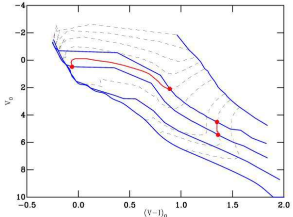
Figure 19. Isochrones (solid blue lines) from Siess et al. (2000) for the approximate ages of the four fields in Figure 18; 1, 3 and 13 Myrs. Mass tracks (dashed lines) are shown for 7, 6, 5, 4, 3, 2, 1.2, 1.0, and 0.8M_{\odot} . The evolution between 1 and 3 Myrs of 3 and 1M_{\odot} stars are shown as filled circles, with the track highlighted in red.
