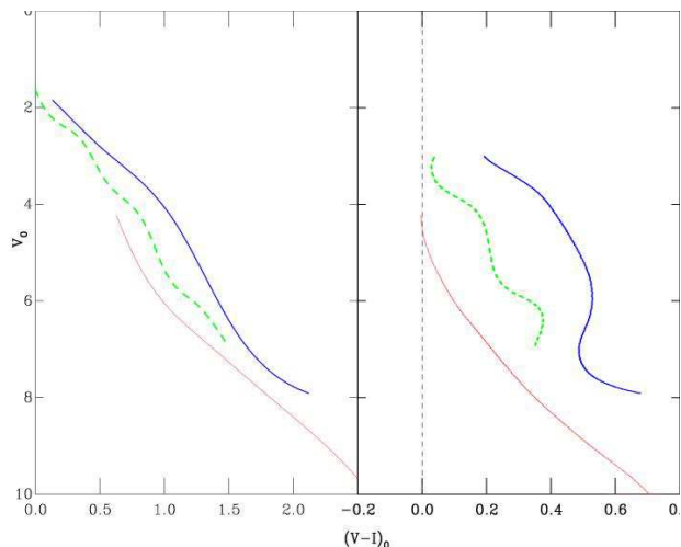
Figure 30. The fitted sequences (solid lines) for (younger to older); NGC7160 (blue, \approx 10 ) and NGC2547 (red, \approx 30-45 Myrs). The dashed line is the spline curve for h and \chi Per ( \approx 13 Myrs). The vertical dashed line shows the position of the ZAMS
