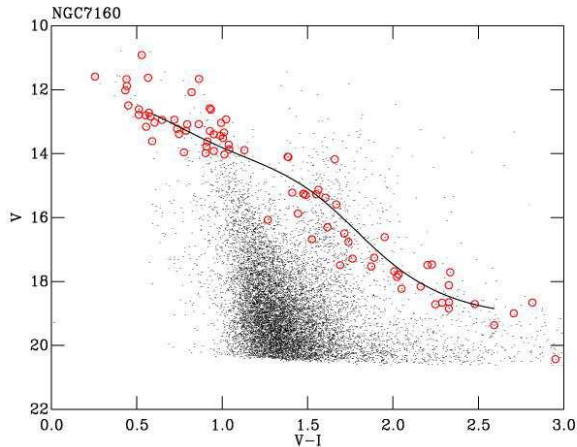
Figure 6. The full catalogue for the NGC7160 field (dots). Circles are members from Sicilia-Aguilar et al. (2004) and Sicilia-Aguilar et al. (2005).
