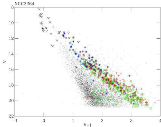
Figure A1. The full catalogue for the NGC2264 field (dots). Circles are the periodic variables from Lamm et al. (2004), asterisks are X-ray sources from Flaccomio et al. (1999) and crosses are H\alpha sources from Dahm & Simon (2005).
