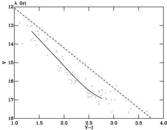
Figure 10. Stars selected as members in \lambda Ori. The dots are Li members from Dolan & Mathieu (2001).
