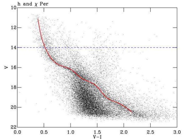
Figure 14. The full catalogue for the h and \chi Per field (dots). The dotted line shows a colour-magnitude selection of V < 14 th, showing the sequence clear of the contamination. The solid line is the best fitting spline to the selected sequence corrected to the mean extinction for the two clusters.
