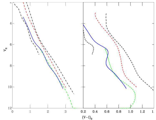
Figure 25. The fitted sequence for IC348 (solid line). h and \chi Per, \sigma Ori, NGC2264 and the ONC are shown as dashed lines for reference.
