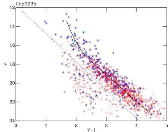
Figure 8. Stars selected as members in Cep OB3b. Asterisks are X-ray sources from Naylor & Fabian (1999), Getman et al. (2006) and the second PSPC catalogue. Triangles are members from Pozzo et al. (2003). Circles are H\alpha sources from Ogura et al. (2002). Crosses are the periodic variables from Littlefair et al (in preparation). The fitted spline curve is shown.
