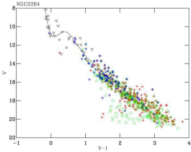
Figure 2. Stars selected as members of NGC2264. Circles are the periodic variables from Lamm et al. (2004), asterisks are X-ray sources from Flaccomio et al. (1999), crosses are H\alpha sources from Dahm & Simon (2005) and triangles are proper motion members from Mendoza V. & Gomez (1980). The spline fit to the sequence after a colour-magnitude selection is shown.
