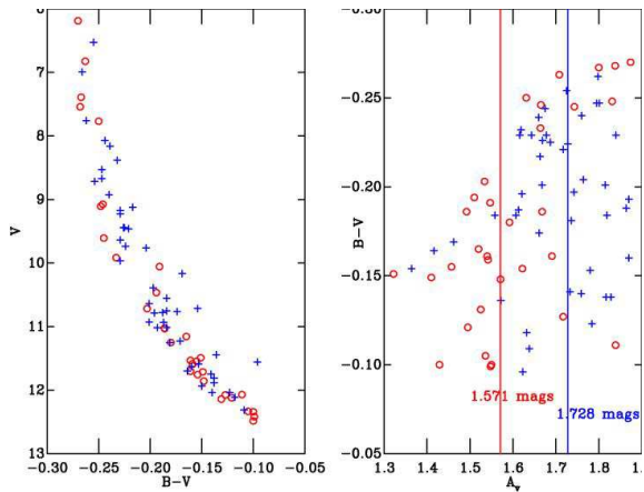
Figure 17. Left. The sequences for h and \chi Per O and B stars after the application of the Q-method. Right. The extinction. The circles are \chi Per and the crosses are h Per. The resulting median values of A_V=1.571 and 1.728 for \chi and h Per respectively are shown.
