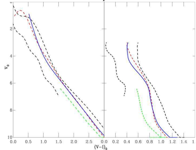
Figure 23. The fitted sequence for Cep OB3b (solid line). NGC2264, h and \chi Per, \sigma Ori, and the ONC are shown as dashed lines for reference.
