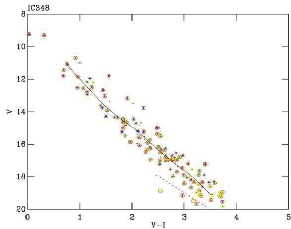
Figure 9. Stars selected as members in IC348. The asterisks are X-ray sources from Preibisch & Zinnecker (2002) and the Second ROSAT PSPC catalogue. Circles are the periodic variables from Cohen et al. (2004) and Littlefair et al. (2005). Crosses are H\alpha sources from Herbig (1998). Triangles are spectroscopic members with extinctions from Luhman et al. (2003) and Herbig (1998). Individual extinctions from Luhman et al. (2003) and Herbig (1998) have been applied before fitting.
