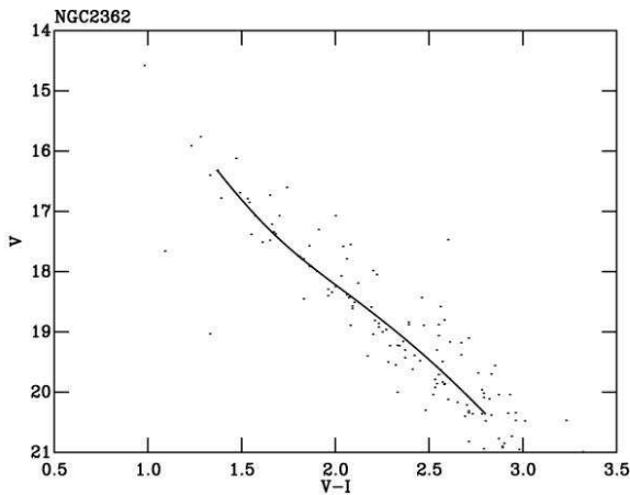
Figure 11. Stars selected as members in NGC2362. The dots are H\alpha and spectroscopically confirmed PMS members from Dahm (2005).
