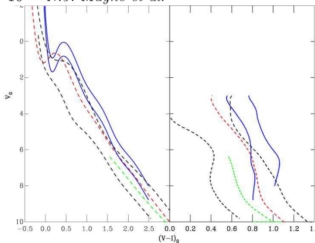
Figure 29. The fitted sequence for NGC6530 (solid line). The ONC, NGC2264, \sigma Ori and h and \chi Per are shown as dashed lines for reference.
