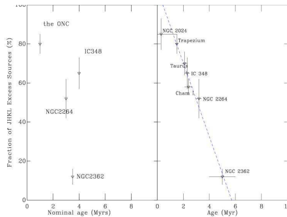
Figure 31. Fraction of JHKL excess sources, used a disc indicator for the ONC, IC348, NGC2264 and NGC2362 from Haisch et al. (2001); left panel, against nominal ages found in this work, right panel, against cluster ages used in Haisch et al. (2001). The straight line is a simple linear regression fit.
