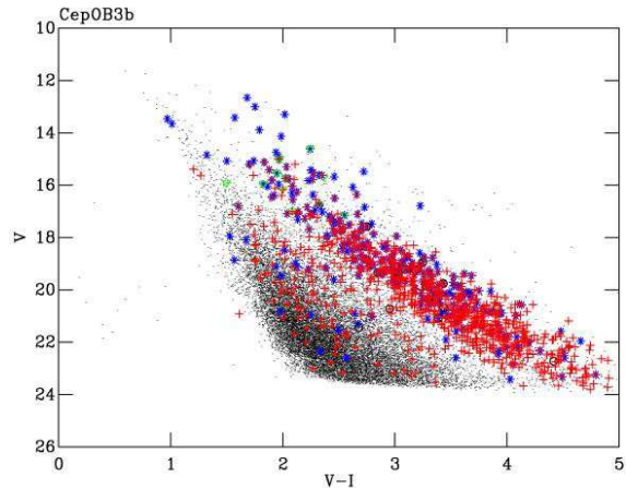
Figure A3. The full catalogue for the Cep OB3b field (dots). Asterisks are X-ray sources from Naylor & Fabian (1999), Getman et al. (2006) and the Second ROSAT PSPC catalogue. Triangles are members from Pozzo et al. (2003). Circles are H \alpha sources from Ogura et al. (2002). Crosses are the periodic variables from Littlefair et al (in preparation).
