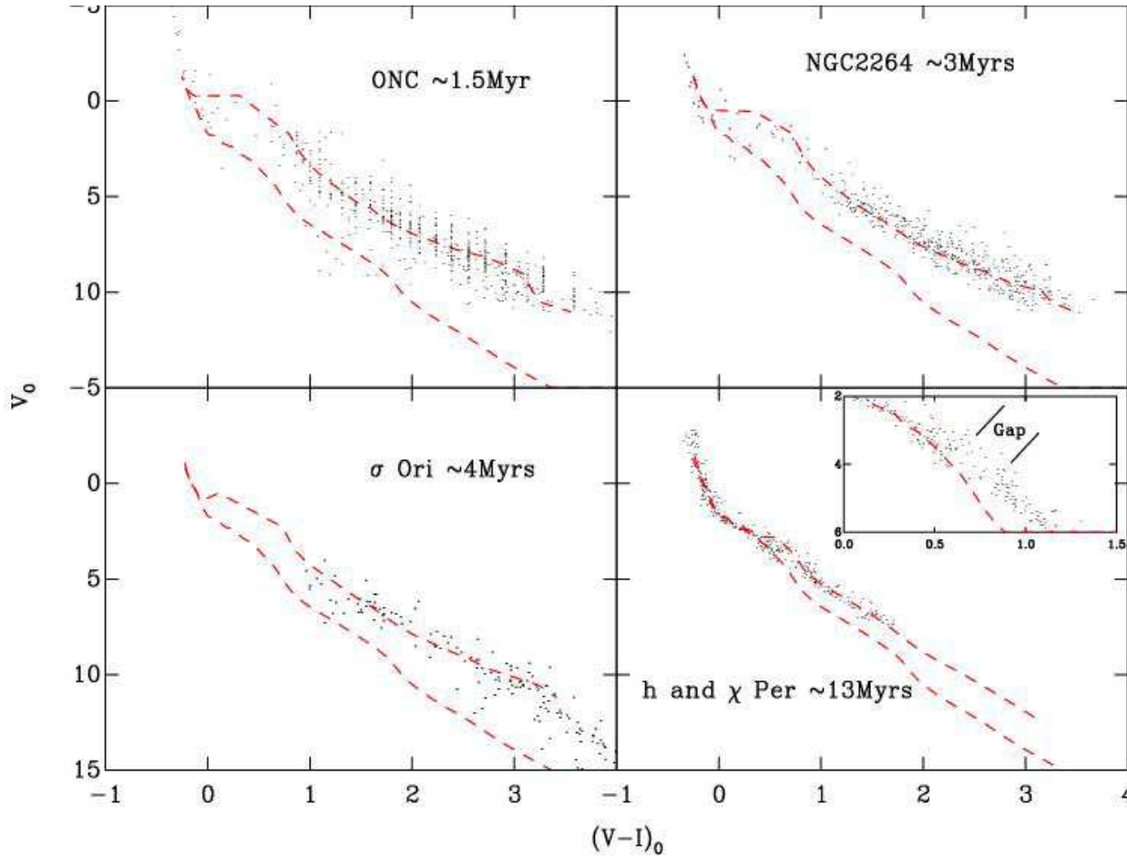
Figure 18. The likely PMS objects for fields of different ages, plotted in dereddened colours and absolute magnitudes. The spread in absolute colour magnitude space clearly decreases as age increases. The ZAMS and isochrones of approximately the correct age from Siess et al. (2000) are shown.
