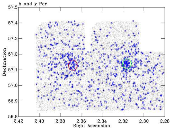
Figure 15. The positions of stars in the h and \chi Per catalogue. Asterisks are stars with V < 14 th, and the large circles show the regions we selected.
