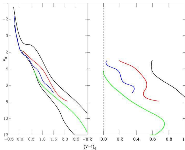
Figure 20. A sample of the empirical isochrones. Youngest to oldest, the ONC, NGC7160, h and \chi Per and NGC2547. The left panel is the empirical isochrones in an absolute V , V-I CMD, with the lowest curve the ZAMS relation of Siess et al. (2000). The right panel is the ZAMS subtracted space; at a given V the ZAMS V-I is subtracted from the V-I of the spline. The vertical dashed line shows the position of the ZAMS
