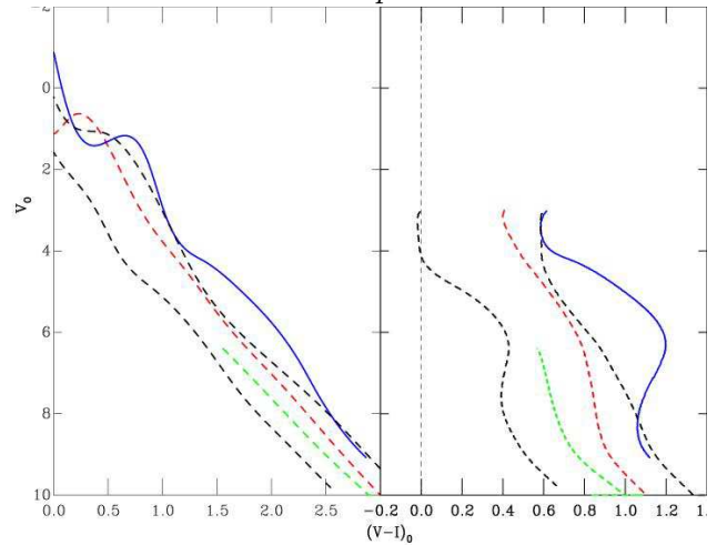
Figure 28. The fitted sequence for IC5146 (solid line), assuming the distance modulus from Herbig & Dahm (2002). The ONC, NGC2264, \sigma Ori and h and \chi Per are shown as dashed lines for reference. The vertical dashed line shows the position of the ZAMS
