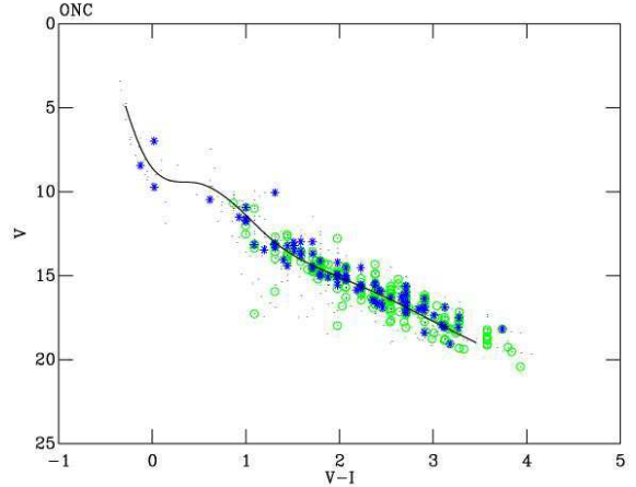
Figure 5. The ONC photometry from Hillenbrand (1997) (dots). Circles are objects which are periodic variables from Herbst et al. (2002). The asterisks are X-ray sources from Flaccomio et al. (2003). The best fit spline through all data points is also shown.
