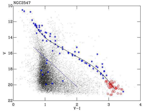
Figure 4. The full catalogue for the NGC2547 field (dots). Asterisks are the X-ray sources from Jeffries & Tolley (1998), circles are spectroscopic members from Jeffries & Oliveira (2005). The X-ray sources, some of which clearly lie in the BG MS contamination were removed using a colour-magnitude cut prior to fitting, shown here as the dotted blue line.
