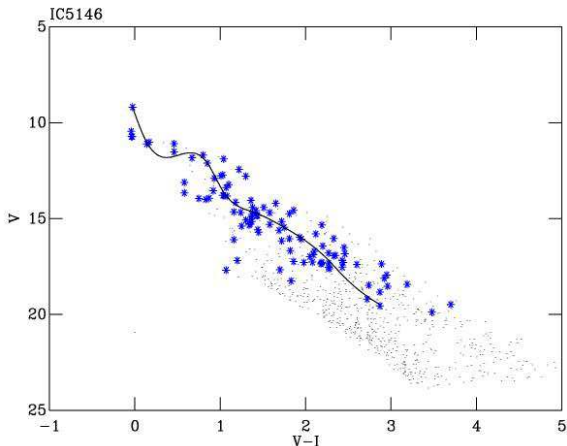
Figure 12. Stars selected as members in IC5146. Dots are likely PMS members from Herbig & Dahm (2002). Asterisks are H\alpha members from Herbig & Dahm (2002) with known spectral types excluding stars lying below the Pleiades MS. Only the asterisks were fitted.
