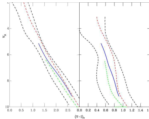
Figure 27. The fitted sequence for NGC2362 (solid line). The ONC, NGC2264, \sigma Ori and h and \chi Per are shown as dashed lines for reference.
