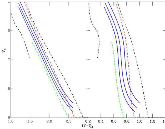
Figure 26. The sequence for \lambda Ori assuming the distance moduli from Dolan & Mathieu (2001), Murlin & Penston (1977) and HIPPARCOS (solid lines). The ONC, NGC2264, \sigma Ori and h and \chi Per are shown as dashed lines for reference.
