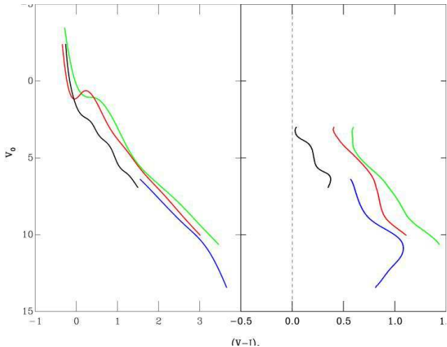
Figure 22. The selected fiducial sequences; h and \chi Per, \sigma Ori, NGC2264 and the ONC. The vertical dashed line shows the position of the ZAMS
