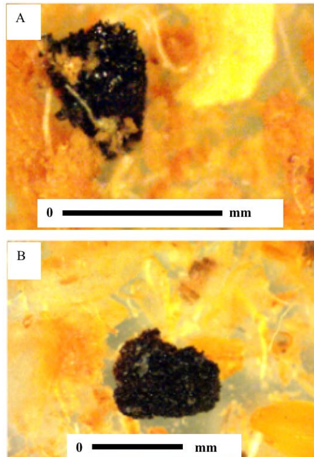
Figure 5. All Saints Bog charred decomposed peat aggregates. Images are from two of the four samples in which evidence of charred peat was found. A: a charred peat aggregate from depth 50–60cm; B: a charred peat aggregate from depth 100–110 cm.
