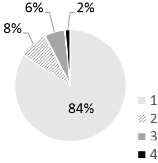
605 606 607 608 Figure 3: Optimisation models (of papers from the appendix table) by: (a) number of objectives, (b) number of constraints, (c) number of types of a decision variable, in an optimisation model
