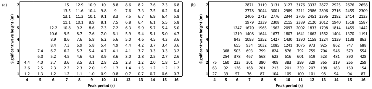
Fig. 3. Power matrices showing absorbed power in kW per sea state bin for hypothetical WEC devices: (a) an offshore bottom-referenced heaving buoy, (b) a nearshore bottom-fixed oscillating flap (from [12]).
