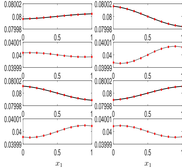
Figure 14: The interface positions h_1(x_1, t) (solid line, upper panels) and h_1(x_1, t) + h_2(x_1, t) (dotted line, lower panels) for the results in figure 4 at, top 2 rows: t = 10 and t = 20 , bottom 2 rows: t = 30 and t = 40 . The dots represent the exact linear solution (C-86) for the lowest frequency mode. The rigid lid is at h_1^0 + h_2^0 + h_3^0 = 0.12 m.
