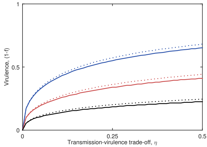
Figure S2 – The evolutionary stable level of virulence obtained using adaptive dynamics (solid curves) and R_0 maximization (dotted). R_0 slightly overestimates the evolutionarily stable level of virulence (as it lacks population structuring), but provides a good approximation for the adaptive dynamics result. Colors correspond to different values of the mate choice parameter, g : g=1/3 (blue); g=1 (red); and g=3 (black). Fixed parameters as in Fig. 2.
