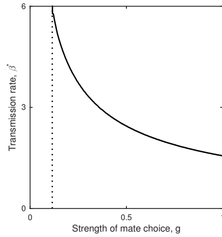
Figure S4 – Optimal values for the transmission rate, \beta , decrease as the strength of mate choice, g , increases. Runaway selection for \beta (and hence virulence) occurs to the left of the dotted line. Fixed parameters as in Fig. 3f.
