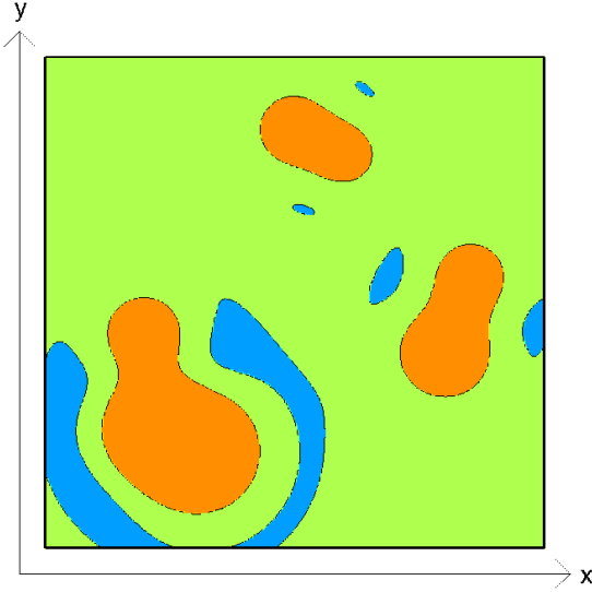
FIG. 1. Schematic horizontal section showing a decomposition of the fluid into multiple components, for example updrafts (orange), downdrafts (blue), and environment (green). In each component one of the I_i is equal to 1 and the others are equal to 0.
