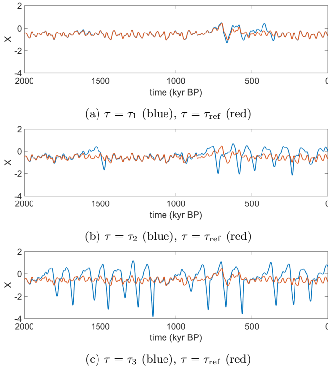
FIG. 5: Trajectories in bistable region (blue) compared to a reference trajectory at \tau_{\text{ref}} = 1.25 (red) for delays (a) \tau_1 = 1.30 , close to homoclinic connection, (b) \tau_2 = 1.45 , middle of bistable region, and (c) \tau_3 = 1.60 , close to Hopf bifurcation. Values of \tau are indicated on bifurcation diagram in Fig. 2a. Other parameters: p = 0.95 , r = 0.8 , s = 0.8 , and u = 0.25 . Initial condition X(t) = -0.5 for t \in [2 + \tau, 2] Myr BP in all cases.
