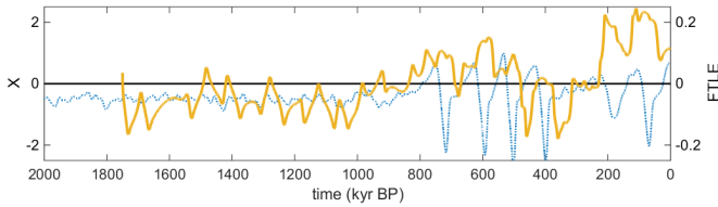
FIG. 8: Finite-time Lyapunov exponents for window length w = 250 kyr computed from model run with \tau = 1.45 and u = 0.15 : X(t) (dotted blue), \text{FTLE}([t - w, t]) (gold).
