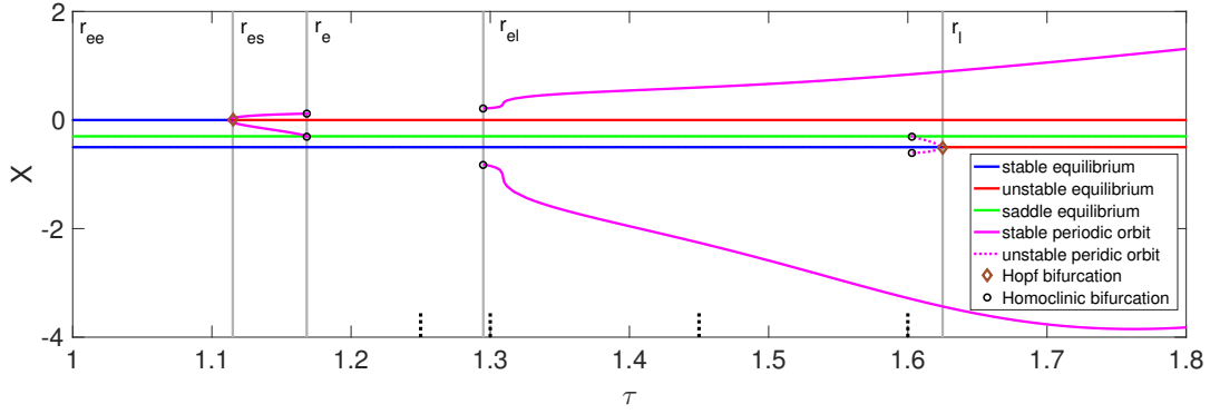
(a) DDE model (4)
