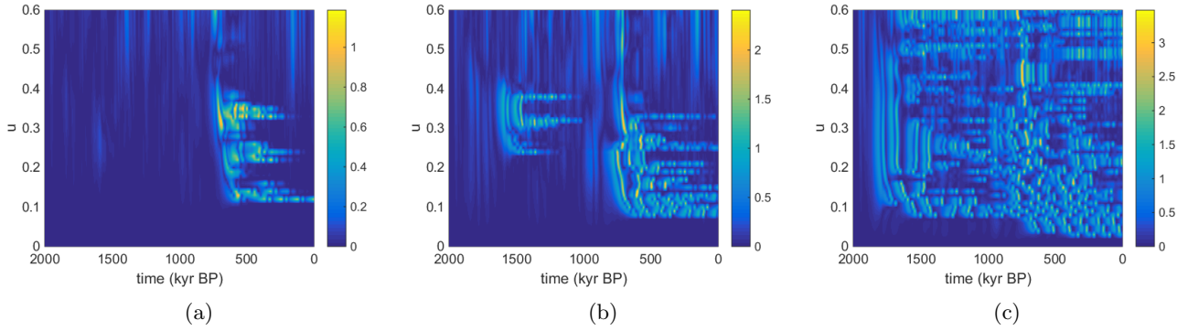
FIG. 6: Distance from reference solution at \tau_{\text{ref}} = 1.25 , for different forcing strengths u . Averages taken over window length of size \tau . (a) \tau = 1.30 , close to homoclinic connection. (b) \tau = 1.45 , middle of bistable region. (c) \tau = 1.60 , close to Hopf bifurcation. Initial condition X(t) = -0.5 for t \in [2 + \tau, 2]\text{Myr BP} in all cases.
