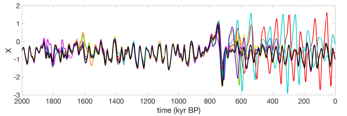
FIG. 12: Trajectories of DDE model with noise: u = 0.45 , \sigma = 0.015 , \tau = 1.45 .
