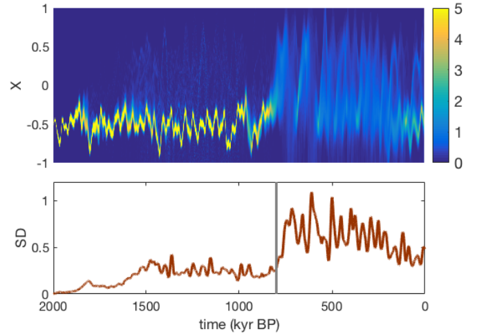
FIG. 11: Probability density in time (top) and its standard deviation (bottom) of 500 model runs with noise: u = 0.15 , \sigma = 0.005 , \tau = 1.45 . The gray line indicates 800 kyr BP
