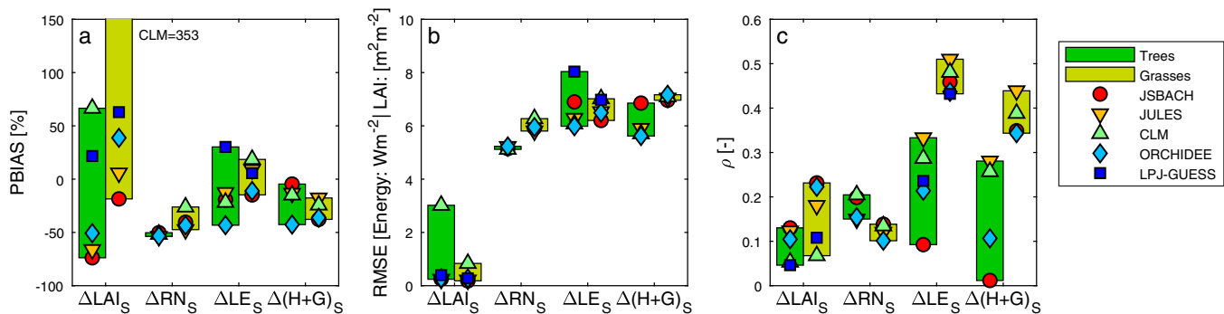
Figure 3. Overall model performance in reproducing single targeted variables. Model performance in simulating single variables, including leaf area index ( \Delta LAI_s ), net radiation ( \Delta RN_s ), latent heat ( \Delta LE_s ), and sensible and ground heat ( \Delta(H+G)_s ). Performance is quantified in terms of (a) percent bias (PBIAS), (b) Root Mean Square Error (RMSE), and (c) Spearman rank ( \rho ). Model-specific performance is visualized with different symbols accordingly to the legend. Intermodel spreads on tree and grass coverages are shown in dark and light green, respectively. Note that the units of measurement of RMSE are different amongst leaf area index and energy fluxes and the PBIAS value of CLM on grasses is out of plot margins.
