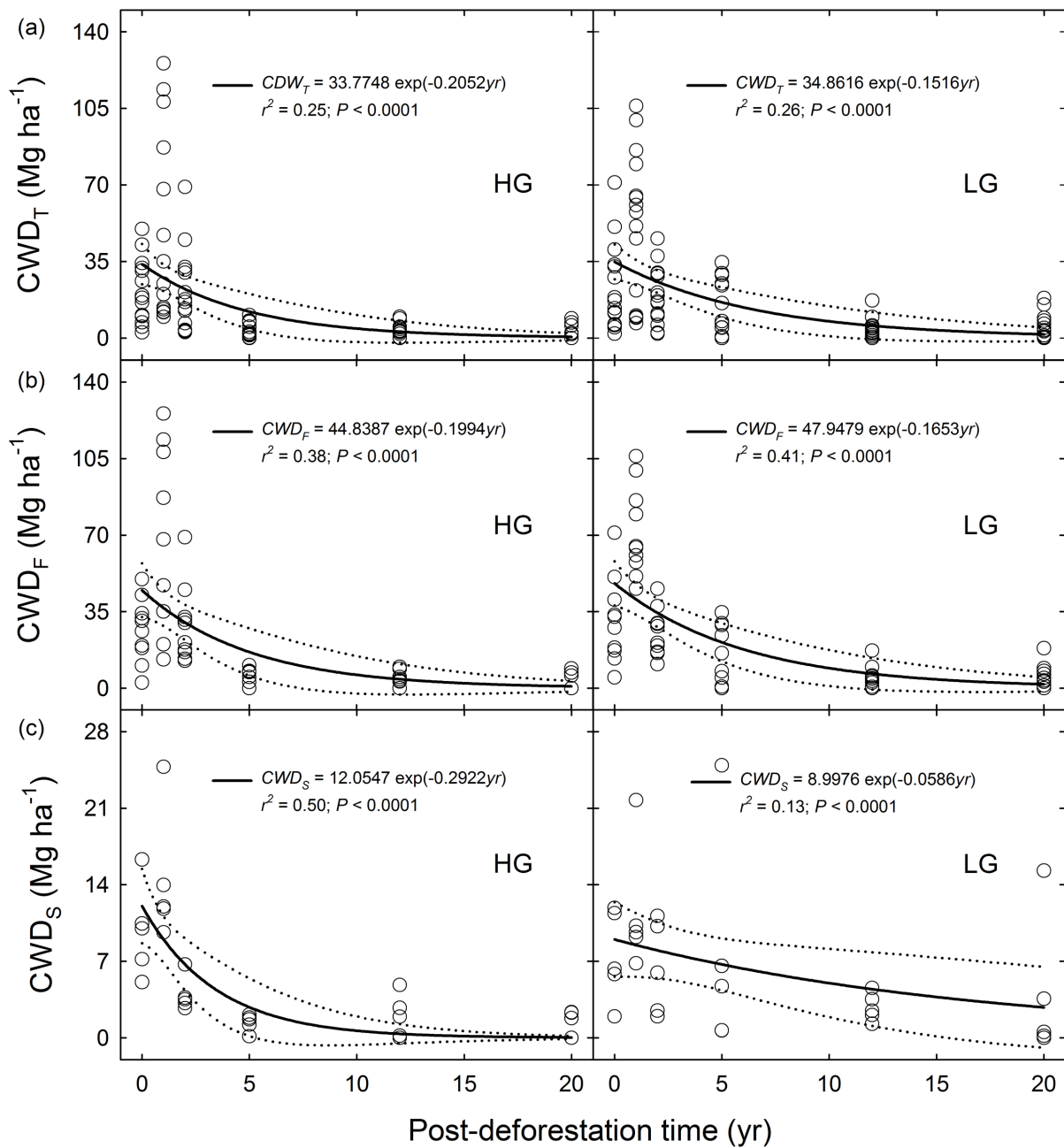
Fig. 4. Dead wood variation of (a) total ( CWD_T ), (b) fallen ( CWD_F ), and (c) standing ( CWD_S ) coarse woody debris during the forest-to-pasture conversion in the high-grazing intensity (HG) and the low-grazing intensity (LG) sub-regions of the Colombian Amazon. The dotted lines represent the 95% confidence interval.
