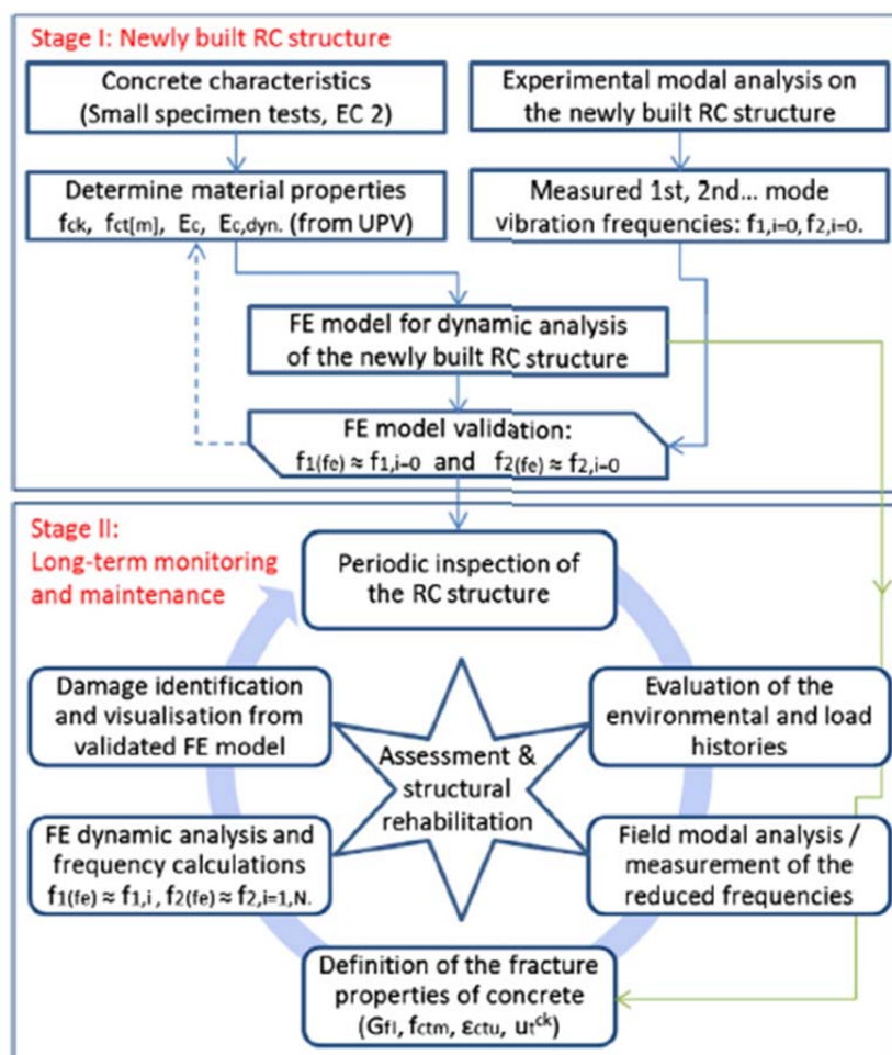
Figure 17: Flow-chart of the initial modal and FE analysis (Stage I) and the long-term structural monitoring, assessment and maintenance cycle that incorporates vibration based damage identification (Stage II).
