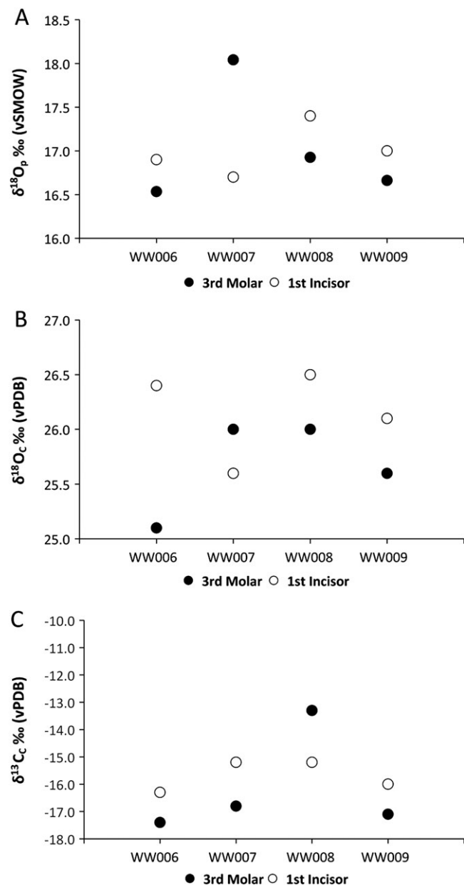
FIGURE 7 The inter-tooth variation in 1 st incisor and 3 rd molar teeth in four individuals from Wytham Woods in (A) \delta^{18}\text{O}_p , (B) \delta^{18}\text{O}_c , and (C) \delta^{13}\text{C} values
