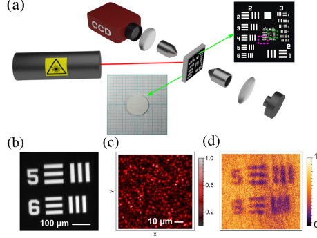
Fig. 1. (a) Experimental apparatus. A cw laser illuminates an opaque scattering material and an object hidden behind (insets). An imaging system records the reflected speckle pattern from the surface of the scattering sample and a bucket detector collects the intensity transmitted by the object. (b) Elements 5 and 6 of Group 4 of the resolution target used as object to image in this experiment, highlighted by the pink square in the inset of panel (a). (c) Typical speckle pattern collected in reflection with the imaging system presented. (d) Retrieved image using BGI with 2.27 \times 10^6 disorder realizations.
