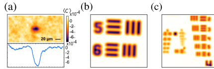
Fig. 3. (a) 2D map and a 1D cross section along \Delta y = 0 of the averaged correlation between the transmitted and reflected speckle patterns. (b) and (c) Expected images obtained by numerically convolving the objects shown in Figs. 2(b) and 2(c) with the correlation function shown in (a).
