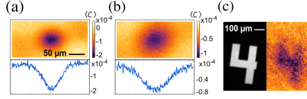
Fig. 4. (a) and (b) Correlation functions between the reflected and transmitted speckle patterns measured 80 \mu\text{m} and 160 \mu\text{m} respectively away from the transmission and reflection surfaces. (c) Object separated by a cover slip of 150 \mu\text{m} from the scattering medium and retrieved image using BGI with 5.65 \times 10^5 disorder realizations.
