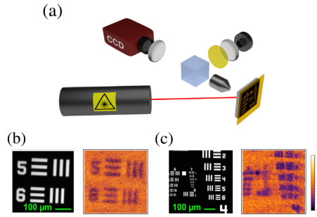
Fig. 2. (a) Experimental apparatus used for non-invasive BGI. A 450 nm laser is incident on the scattering sample at \approx 45^\circ . The resolution target is placed on the back surface of the scattering material, and right behind it we have a fluorescent layer (Cerium-doped YAG), acting as a fluorescent object. The bucket detector is in this case also in reflection from the sample, filtering the fluorescent light with a 500 nm long pass filter. (b) Elements 5 and 6 of Group 4 of the resolution target used as the object, and the image retrieved using BGI with 4 \times 10^6 disorder realizations. (c) Object representing Groups 5, 6 and 7 from the resolution target, and the image retrieved using BGI with 1.5 \times 10^6 disorder realizations.
