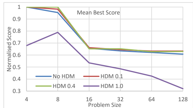
Figure 12: Mean Best Score as problem size increases. The problem size axis uses a base 2 logarithmic scale.
