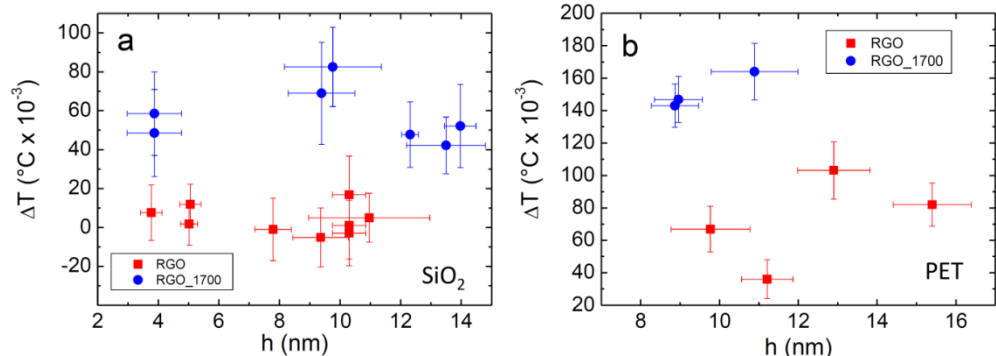
Figure IX.33. (a) Summary of T difference between Si/SiO 2 and RGO (red) or RGO_1700 (blue). (b) The same as in (a) but for PET substrate. Adapted from [334], with permission from Elsevier.
