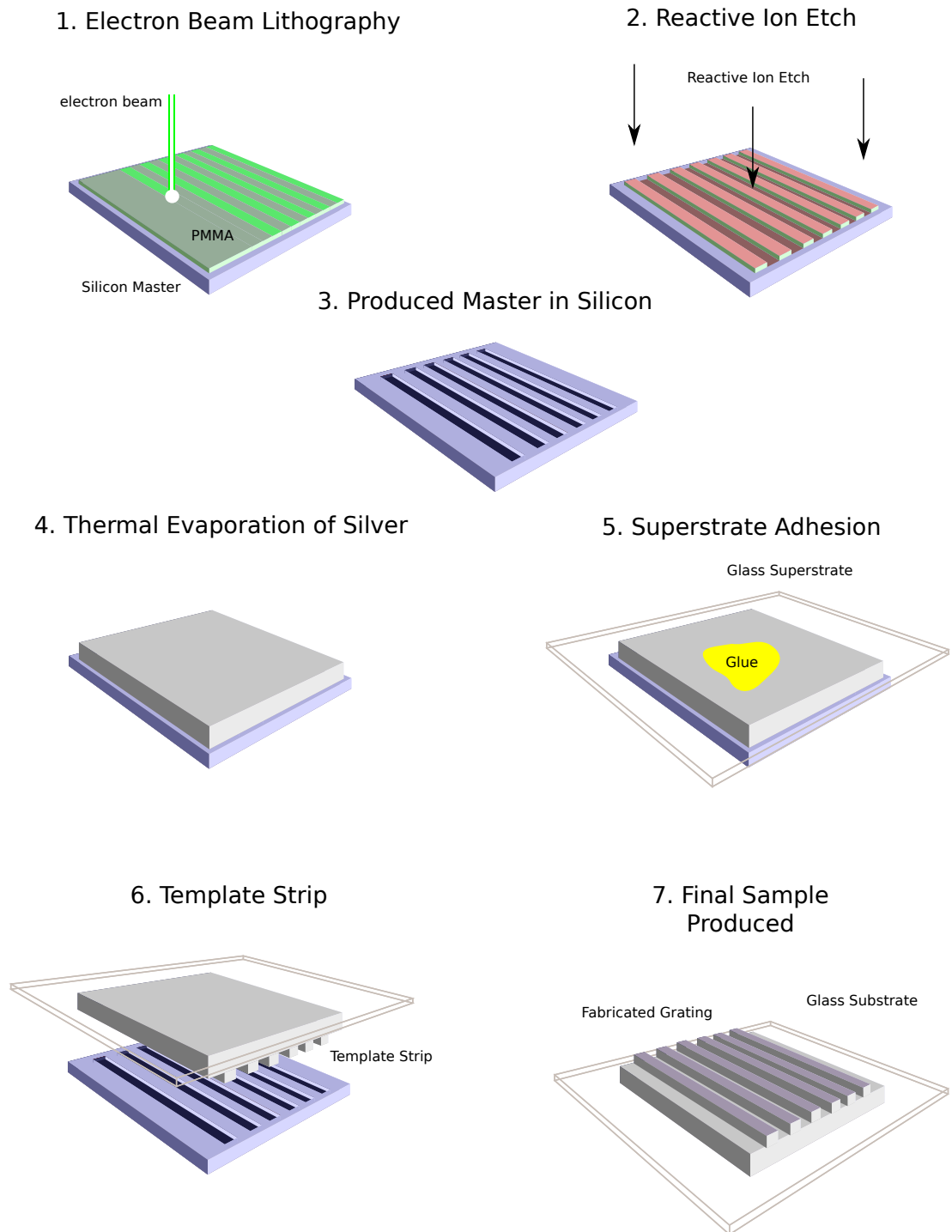
Figure 4.1: Illustration of the fabrication method used for the production of diffraction gratings.
