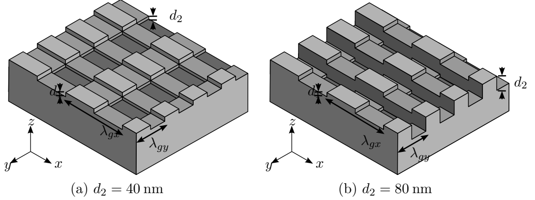
Figure 5.9: Diagram of the effect on the surface profile by increasing the depth d_2 of the rectangular bigrating from (a) d_2 = 40 nm to (b) d_2 = 80 nm. A larger value of d_2 increases the diffraction efficiency of the constituent \mathbf{k}_{gy} grating.
