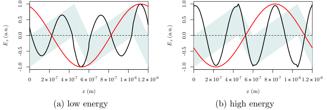
Figure 8.16: The (a) low energy and (b) high energy x -component of the SPP standing wave electric field (black, E_{SPP} ) and incident field (red, E_x ) varying across two unit cells of the asymmetric zigzag grating (light grey shapes indicate the zigzag in the xy plane).
