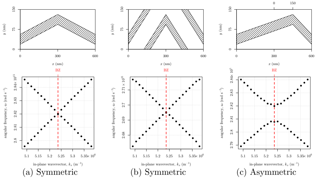
Figure 8.12: The calculated eigenmodes for the crossing of the -1\mathbf{k}_{gx} and +2\mathbf{k}_{gx} scattered SPPs at the first BZ for the cases of: (a) a symmetric zigzag; (b) a symmetric, high-amplitude zigzag and; (c) an asymmetric zigzag. The unit cell for each is shown above the modelled dispersion plots.
