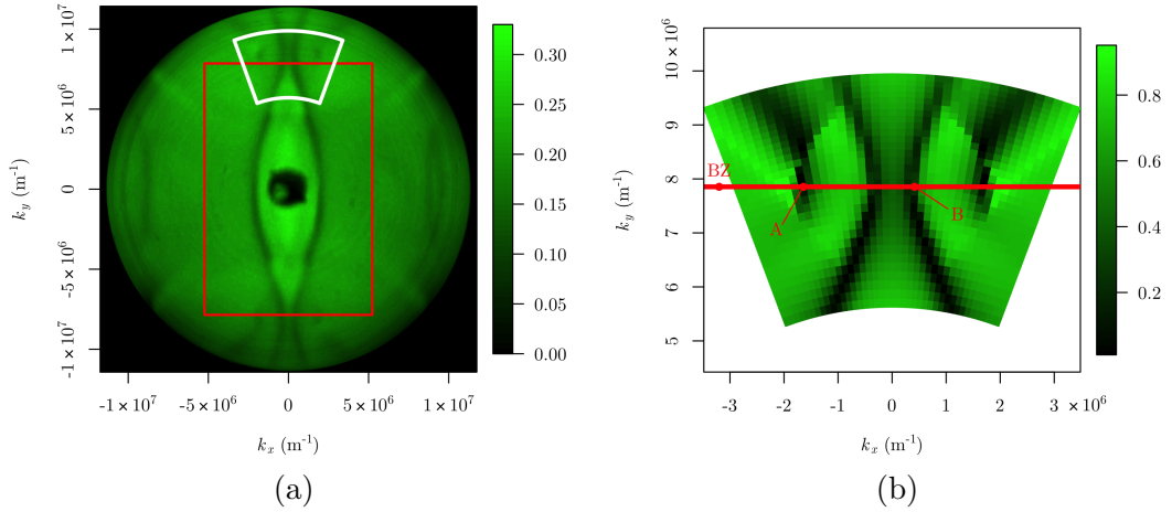
Figure 5.5: (a) A scattergram of a rectangular grating mapped to k -space for an illumination wavelength of \lambda_0 = 550 nm. The red square indicates the position of the BZ boundary. The white region bounded in the scattergram is replicated in (b), modelled using the FEM.
