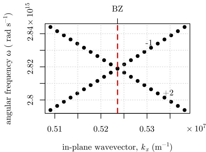
Figure 7.17: Modelled SPP dispersion around the intersection point of the -1\mathbf{k}_{gx} and +2\mathbf{k}_{gx} scattered SPPs meeting at the first BZ boundary (red dashed line).
