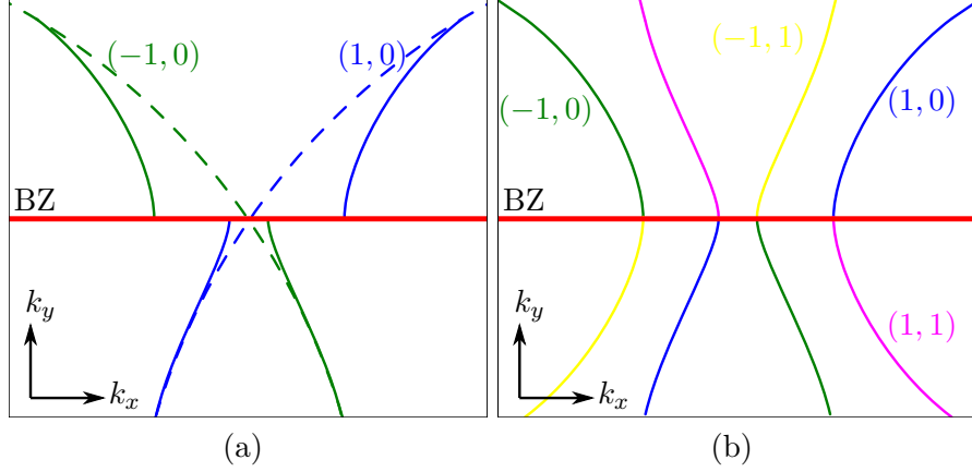
Figure 5.6: (a) Cartoon of the (-1, 0) and (1, 0) SPP iso-frequency contours at the BZ boundary, from the original continuous SPP contours (dotted lines) to the split modes (solid lines). (b) By considering the other interactions occurring at this point (or by using the mirror symmetry of the BZ boundary), the continuous SPP contours are recovered, leading to the observation of the SPP contour shape measured in figure 5.5.
