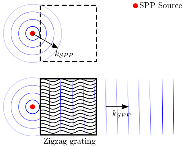
Figure 9.1: A possible experimental arrangement for the observation of collimated surface waves using zigzag gratings.
