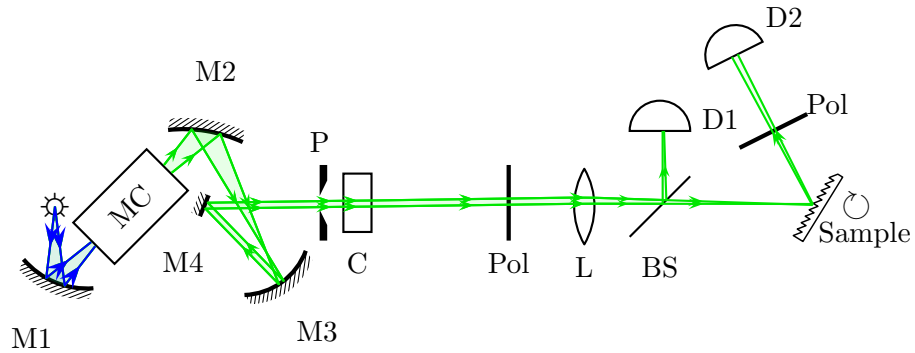
Figure 4.2: System for the measurement of the reflectivity of a sample as a function of both wavelength, \lambda_0 and polar angle \theta . White light is represented as blue lines, pseudo-monochromatic light is shown as green lines.
