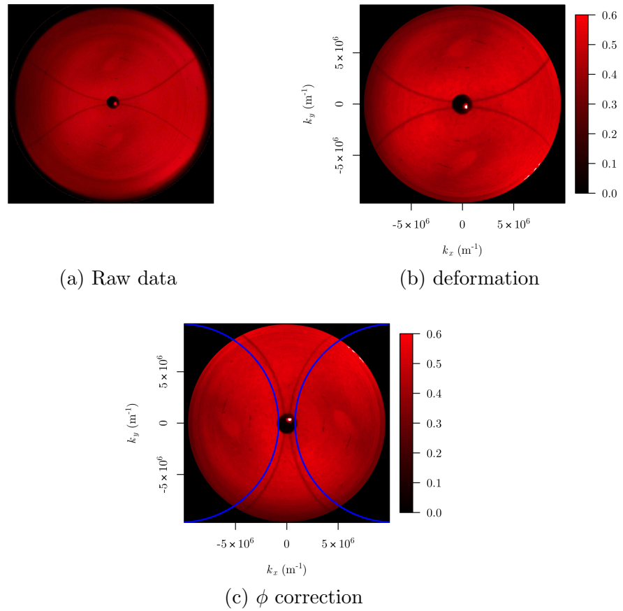
Figure 4.9: The processing of a raw dataset from the scatterometer at a wavelength of \lambda_0 = 650 nm. (a) Raw image obtained from scatterometer, (b) the image after the applied momentum-space deformation, and (c) the final image with corrected azimuthal angle and addition of calculated diffraction circles.
