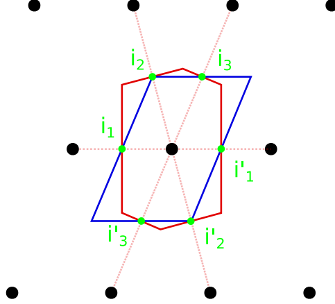
Figure 6.9: Two possible Brillouin Zones for an oblique lattice. The Wigner-Seitz cell (red) and a simple trapezium (blue) contain on their boundaries the points of high symmetry labelled i_1, i_2, i_3 .
