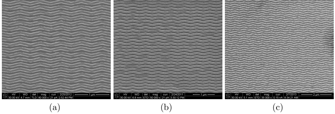
Figure 7.5: Scanning electron micrographs of: (a) an example template-strip master in Si, used for production of zigzag gratings; (b) a polymer replica of a Si master prior to metallisation, for zigzag gratings embedded in glass; (c) a template stripped sample in silver.
