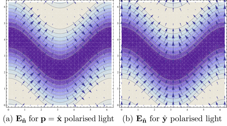
Figure 7.2: The surface normal components of electric field vector for (a) TM and (b) TE polarised light (arrows) projected on a contour of the zigzag surface profile. The contour plot amplitude ranges from 1 (white) to -1 (blue).
