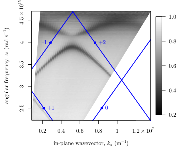
Figure 8.10: The dispersion of the SPP modes mapped as a function of unpolarised light reflectivity on an asymmetric zigzag grating. The blue lines are the calculated positions of the diffracted light lines. The colour scale indicates the absolute reflectivity.
