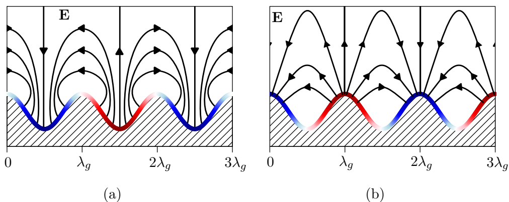
Figure 2.11: Cartoon of two possible SPP standing waves on a sinusoidal grating. The blue and red regions show accumulation of positive and negative charge density, respectively. These two standing waves, both which have a period of 2\lambda_g , result in different field arrangements and so are associated with different energies.
