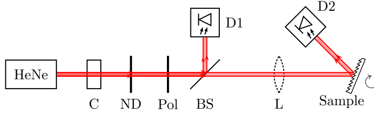
Figure 4.3: System for the measurement of angular dependant reflectivity at a set wavelength of \lambda_0 = 632.8 nm
