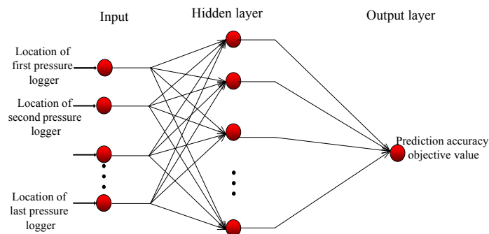
Figure 2. ANN Architecture
