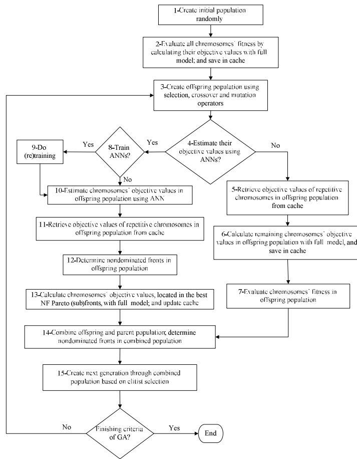
Figure 1. MOGA-ANN Flowchart
