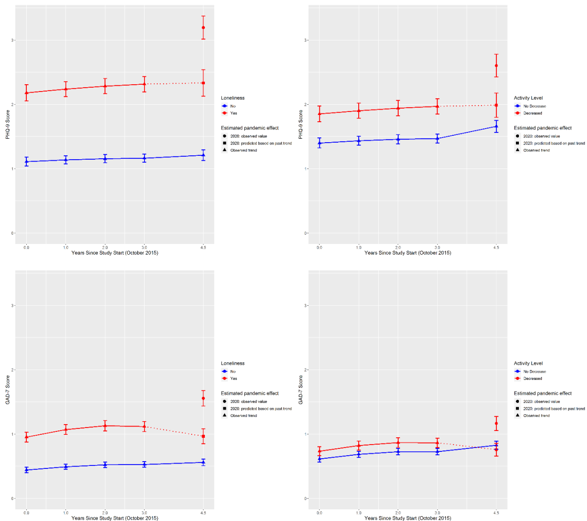
Figure 1A and B Trajectories of predicted PHQ-9 and GAD-7 scores from zero-inflated negative binomial regression models for loneliness and physical activity
