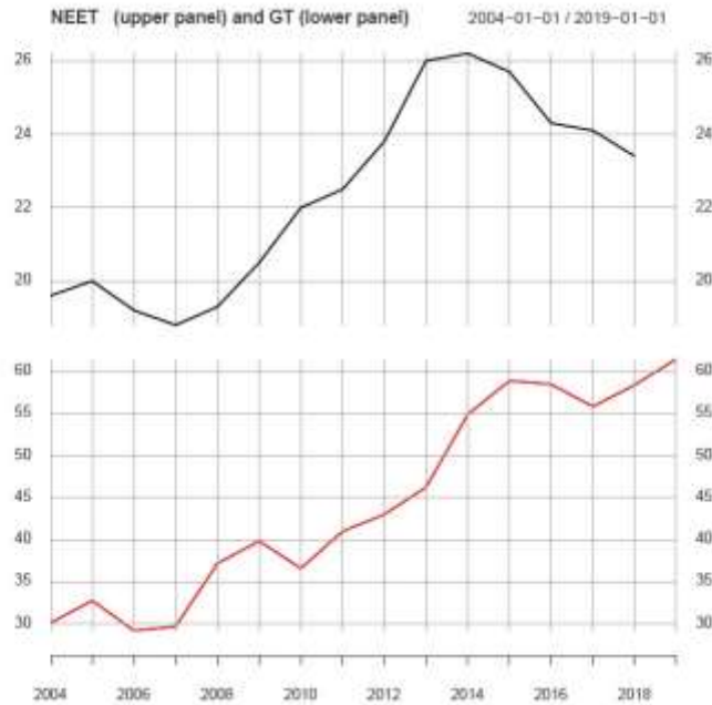
Figure 1. NEETs time series (upper panel) from 2004 to 2018 and GT (lower panel) time series from 2004 to 2019
