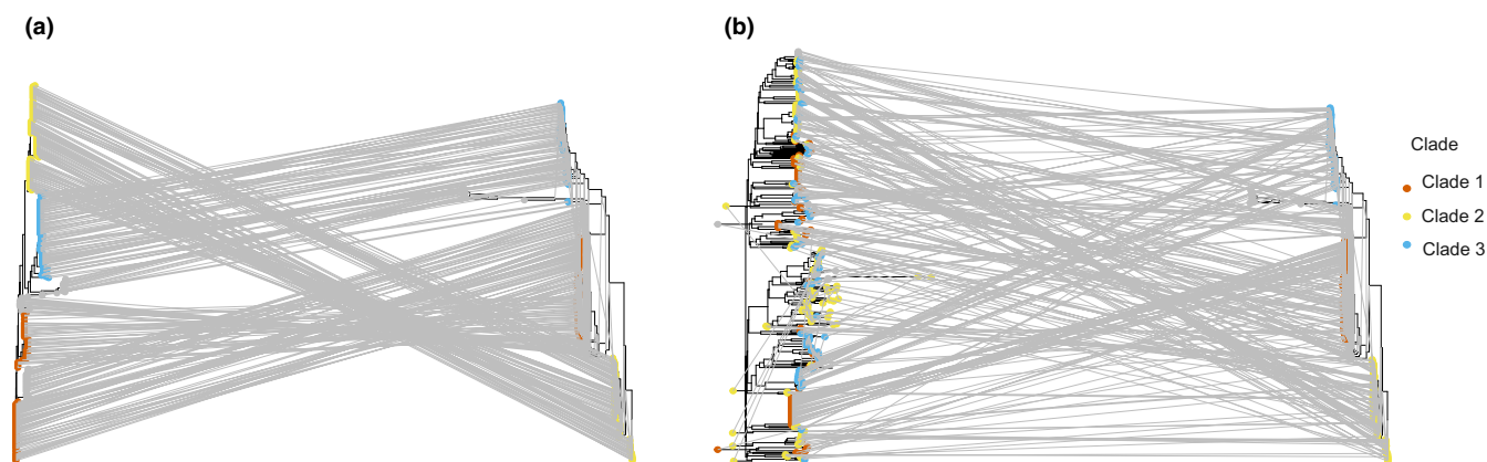
FIGURE 4 Consistency between phylogenies based on a single gene and a core genome. (a) Consistency between the conserved cold shock protein ( CspA ) gene phylogeny and the strict core genome ( n = 1,004 ) of the Bacillus cereus sensu lato ( Bc sl ) group. A given isolate in each tree is connected to the same isolate in the other tree by a line. (b) Consistency between the diverse flagellin ( hag ) gene phylogeny and the strict core genome ( n = 1,004 ) of the Bc sl group. A given isolate in each tree is connected to the same isolate in the other tree by a line
